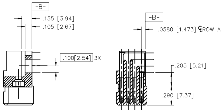
SECTION U-U
