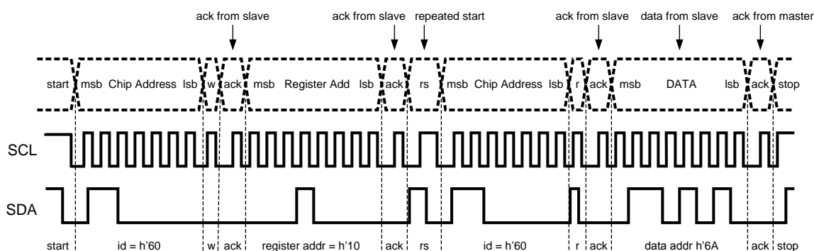
Figure 64. I 2 C Read Cycle
