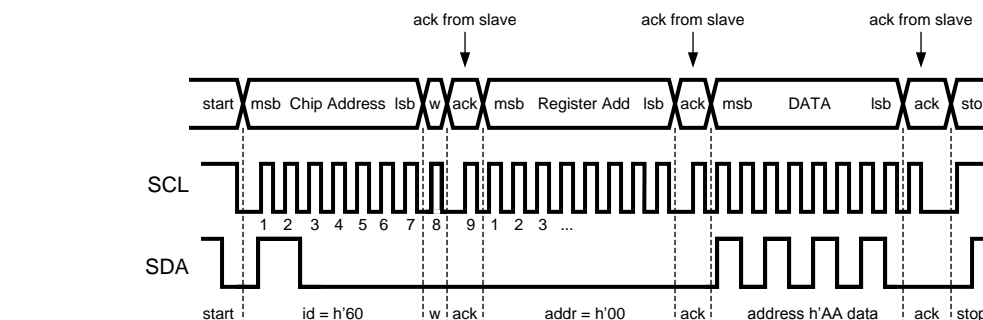
Figure 63. I 2 C Write Cycle
