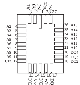
28-Pin Flat Pack (F)
