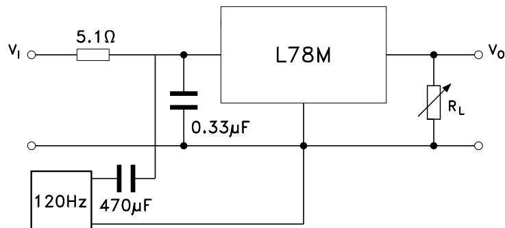
Figure 7. Ripple rejection
