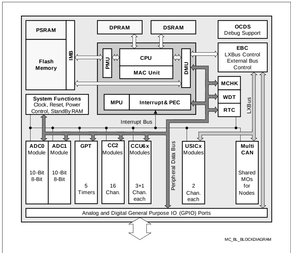
Figure 4 Block Diagram
