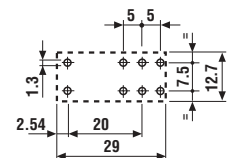
Copper side view
