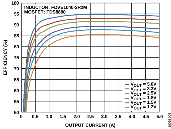
Figure 5. Efficiency at V_{IN} = 12\text{ V} , f_{SW} = 600\text{ kHz} , FPWM
