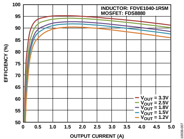
Figure 7. Efficiency at V_{IN} = 5\text{ V} , f_{SW} = 600\text{ kHz} , FPWM
