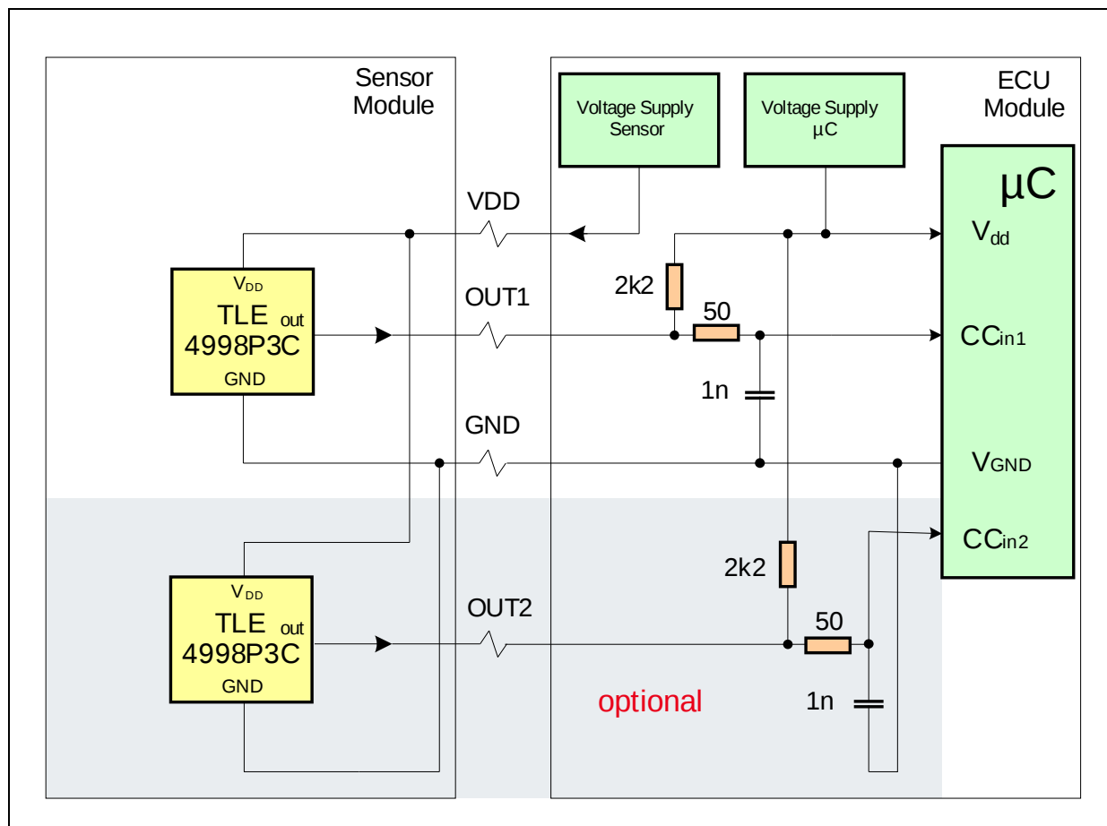
Figure 9 Application Circuit
