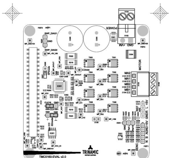
Assembly Drawing Top
