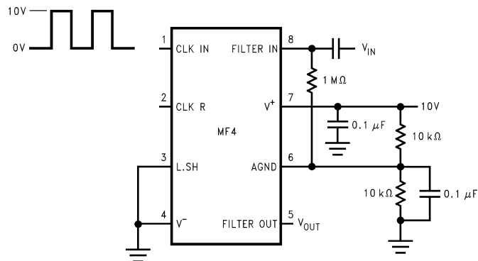
FIGURE 4. Single Supply Operation. ANGND Resistor Biased to V^+/2
