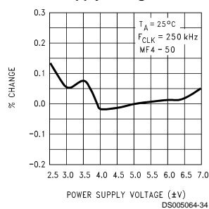
f_{\text{CLK}}/f_c Deviation vs Power Supply Voltage
