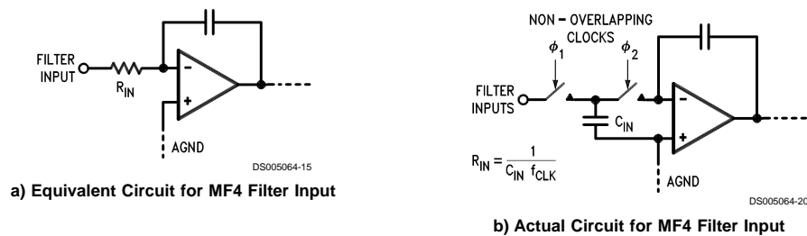
FIGURE 5. MF4 Filter Input
