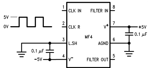
FIGURE 3. Split Supply Operation with TTL Level Clock
