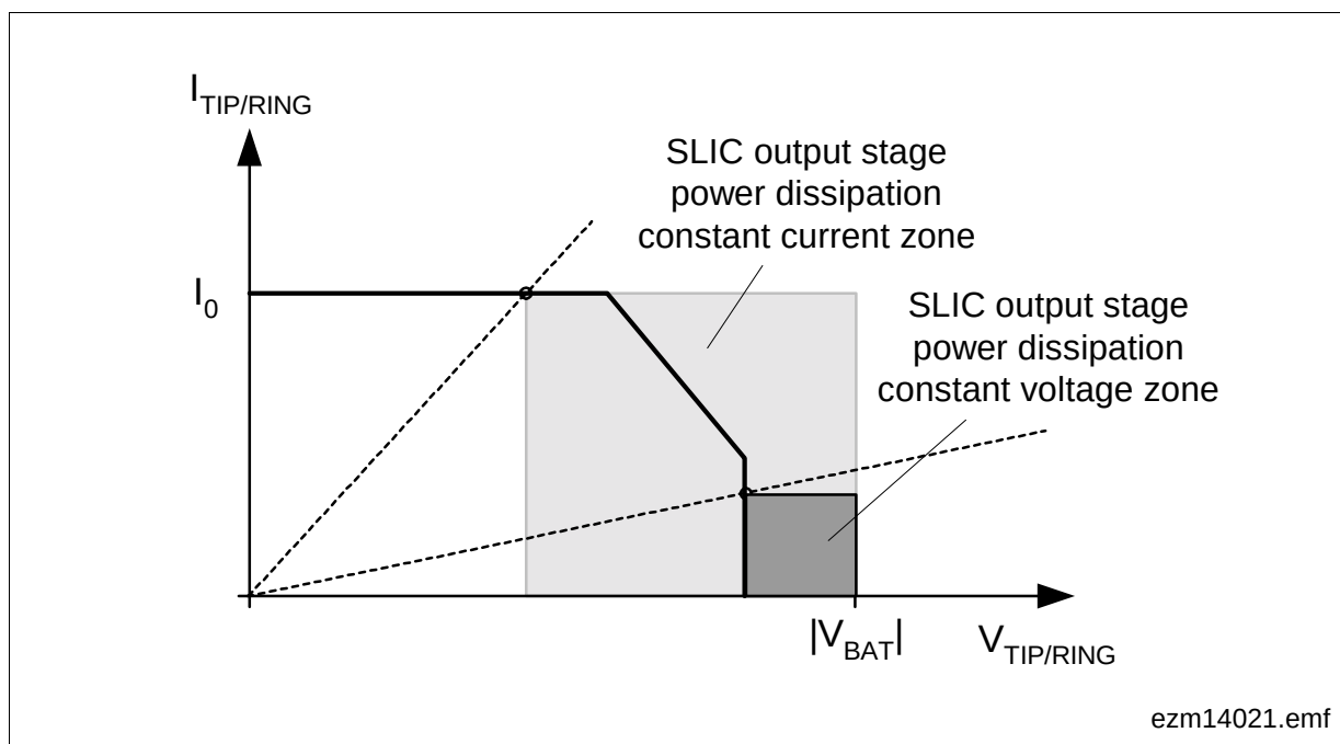
Figure 19 Power Dissipation
