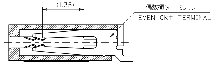
SECT. G-G
