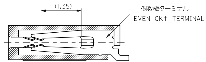
SECT. G-G
