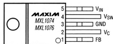
5-PIN TO-220
