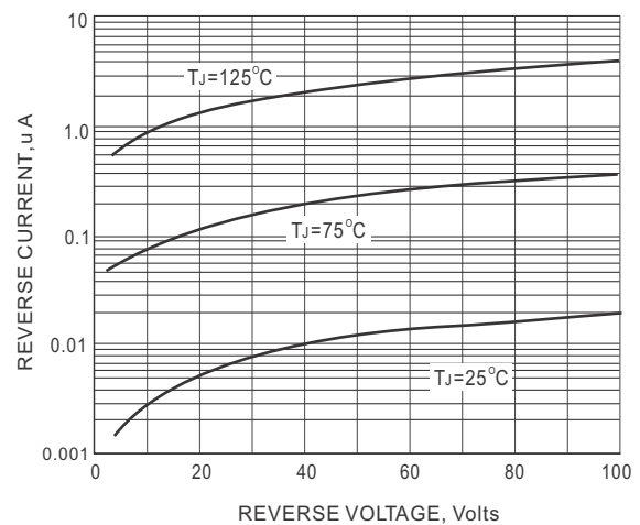
FIG. 2-TYPICAL REVERSE CHARACTERISTICS
