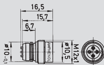
Male panel connector, installation version
