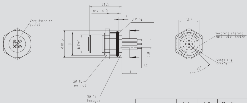
Male panel connector, rear mounting pcb-mount type
