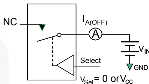
Figure 7. Off Leakage
