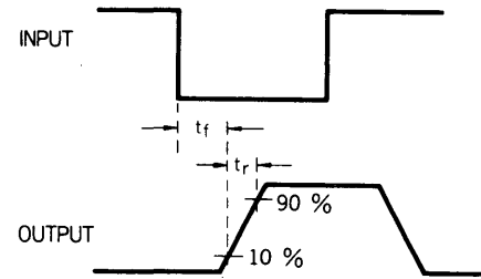
VOLTAGE WAVEFORMS
