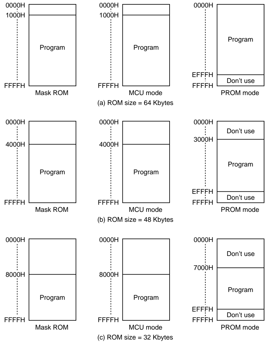
Figure 19-1 Program Memory Area
