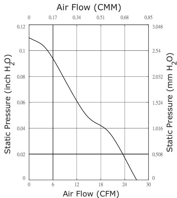
CFM-7015V-133-315
