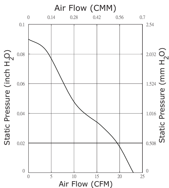
CFM-7015V-128-265
