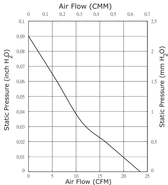
CFM-7020V-126-260
