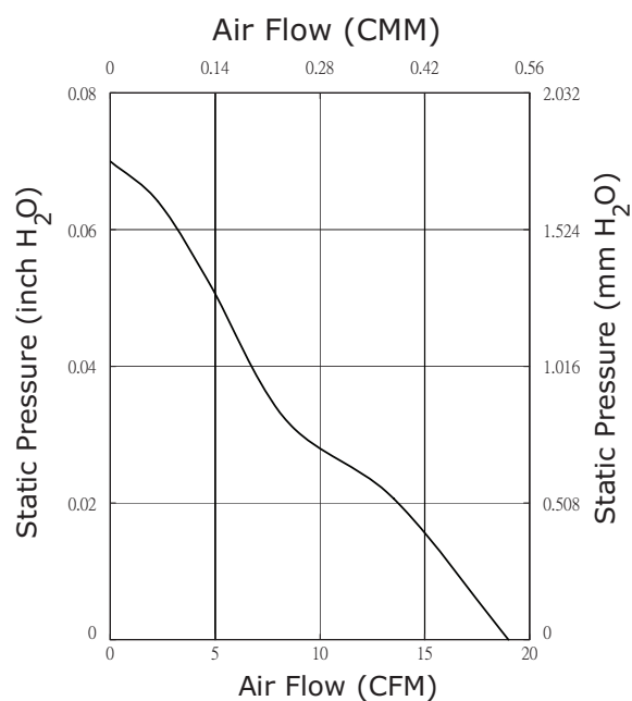
CFM-7015V-123-215
