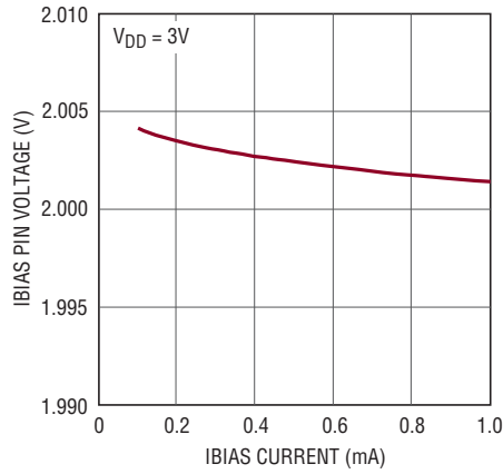
IBIAS Voltage Load Regulation
