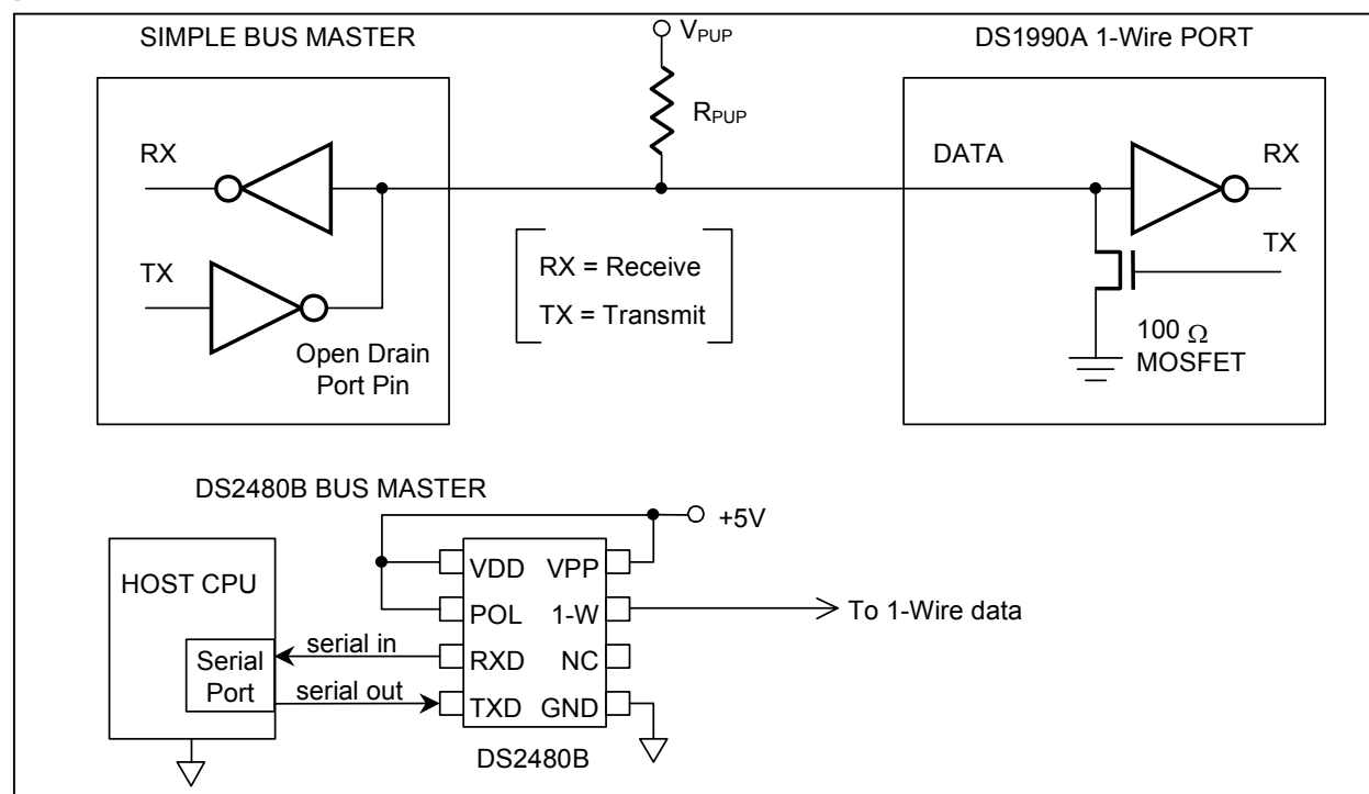
Figure 4. HARDWARE CONFIGURATION
