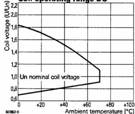
Coil operating range DC
