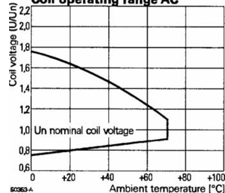
Coil operating range AC
