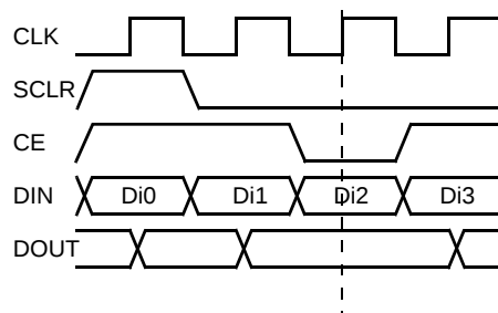
Figure 10: CE and SCLR Timing
