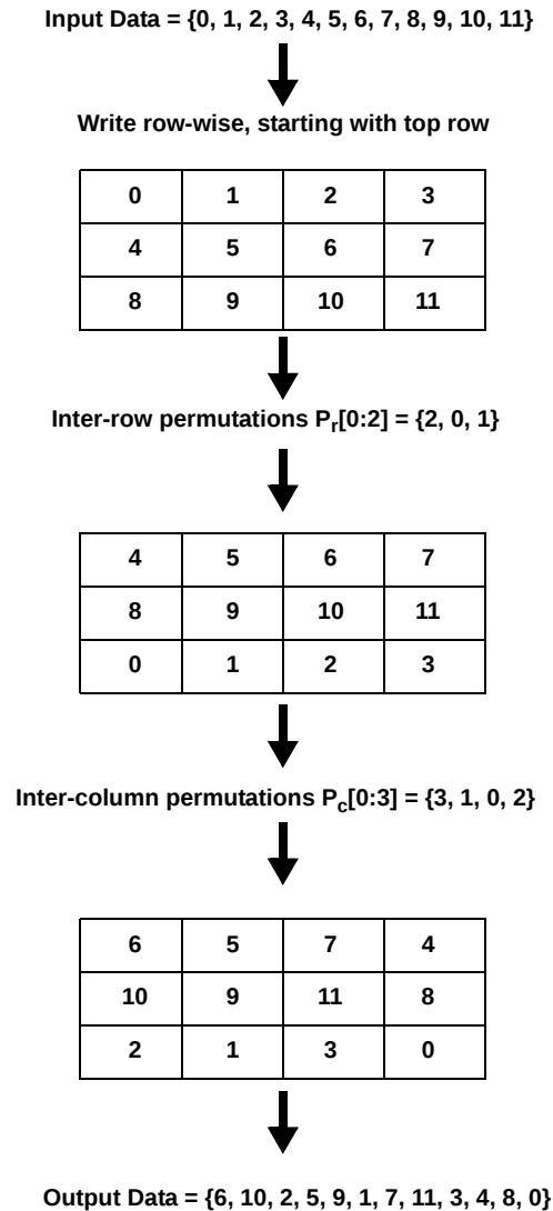
Figure 6: Block Interleaving Example with Row and Column Permutations
