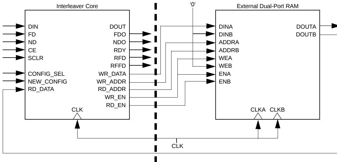
Figure 22: Connections to External Symbol RAM for Convolutional Interleaver
