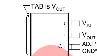
DD PACKAGE (3-PIN) (Top View)
