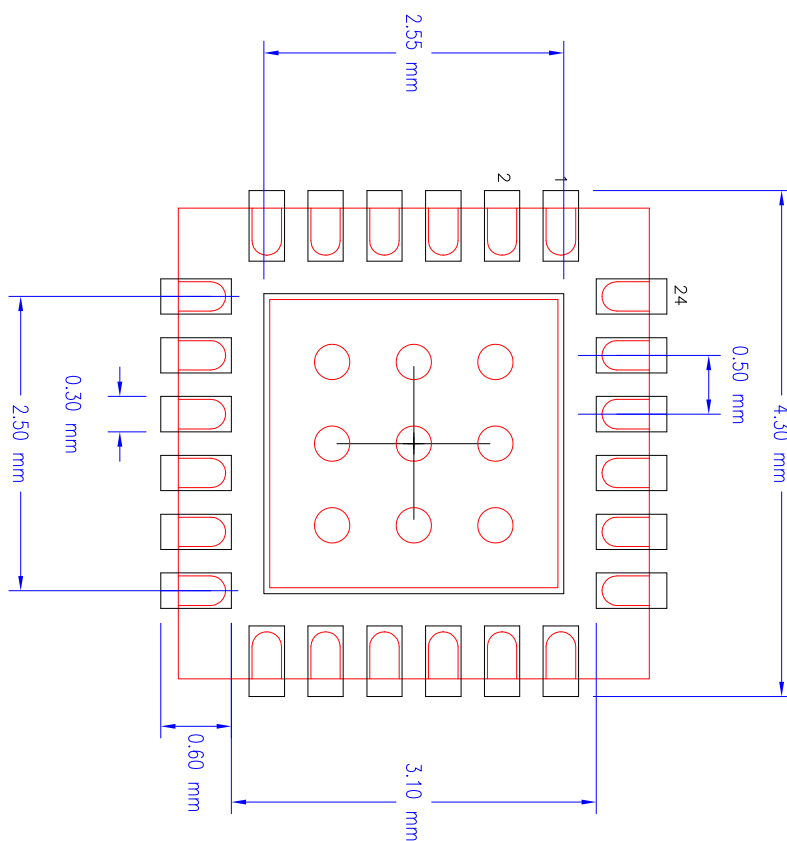
NL24 RECOMMENDED FOOTPRINT 2.45 mm SQ EPAD
