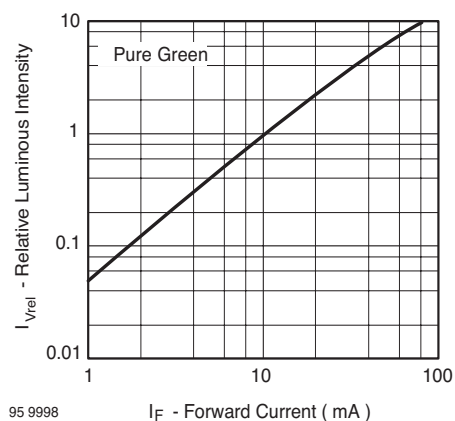
Figure 27. Relative Luminous Intensity vs. Forward Current
