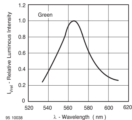
Figure 23. Relative Intensity vs. Wavelength
