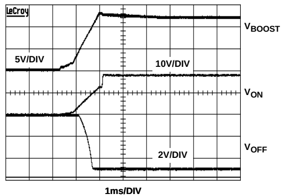
FIGURE 16. POWER-UP
