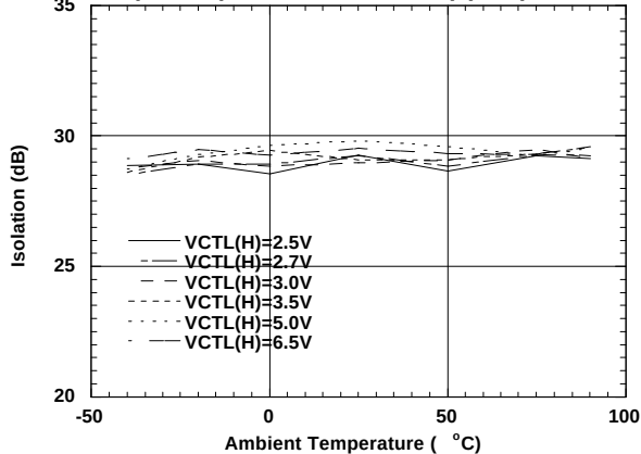
Isolation vs. Ambient Temperature
