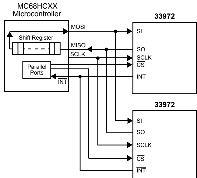
Figure 9. SPI Parallel Interface with Microprocessor
