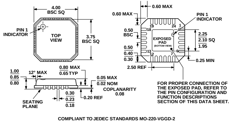
Figure 26. 24-Lead Lead Frame Chip Scale Package [LFCSP_VQ] 4 mm x 4 mm Body, Very Thin Quad (CP-24-1) Dimensions shown in millimeters
