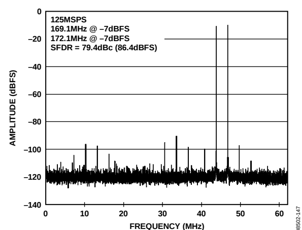
Figure 47. AD9265-125 Two-Tone FFT with f_{IN1} = 169.1 MHz and f_{IN2} = 172.1 MHz
