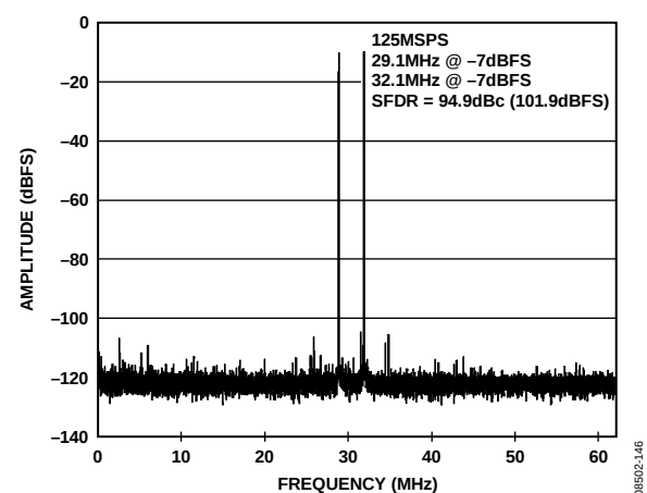
Figure 46. AD9265-125 Two-Tone FFT with f_{IN1} = 29.1 MHz and f_{IN2} = 32.1 MHz
