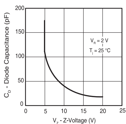
Diode Capacitance vs. Z-Voltage
