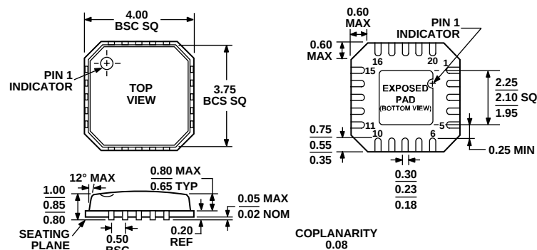
Figure 31. 20-Lead Lead Frame Chip Scale Package [LFCSP_VQ] 4 mm × 4 mm Body, Very Thin Quad (CP-20-1)
