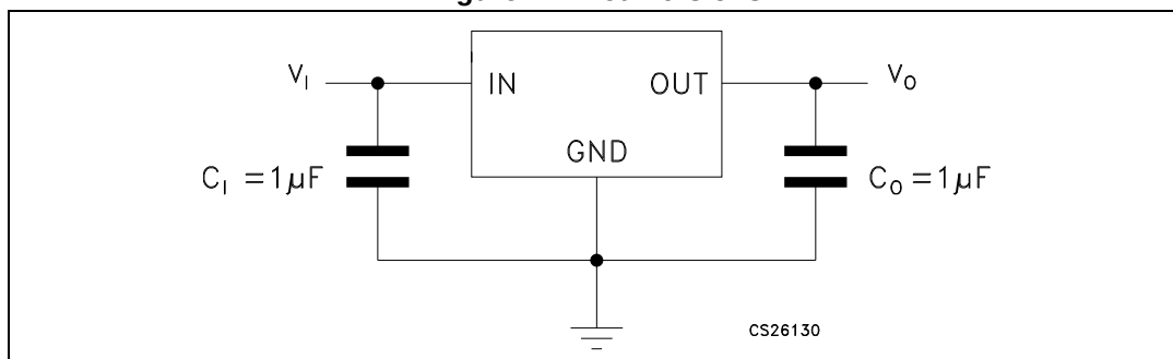
Figure 4. Fixed versions
