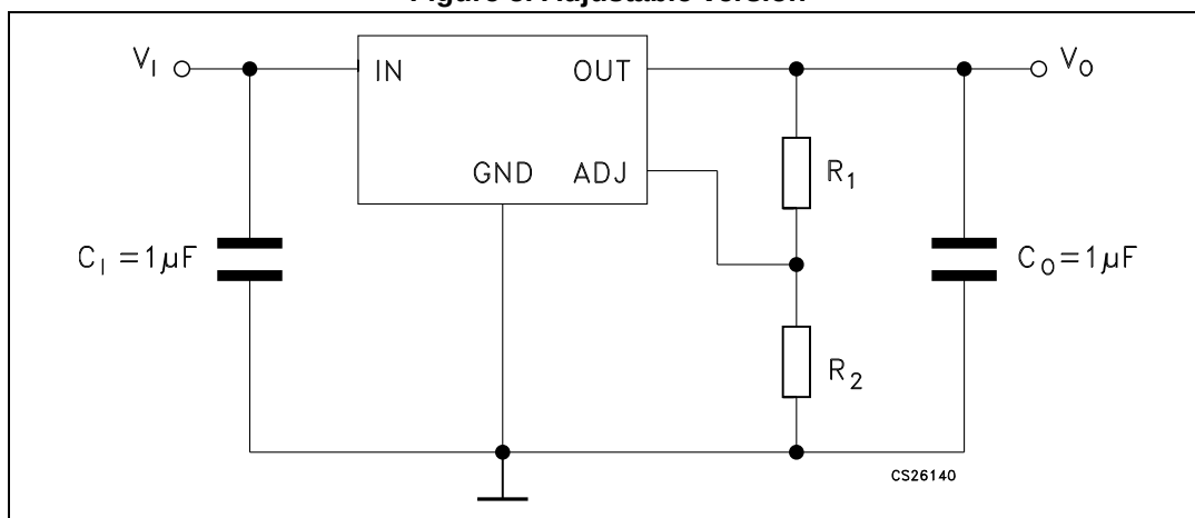
Figure 5. Adjustable version
