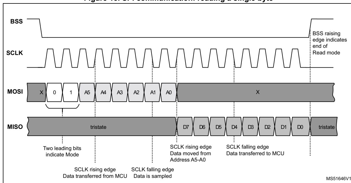
Figure 15. SPI communication: reading a single byte
