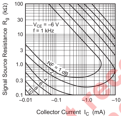
Contours of Constant Noise Figure (3)
