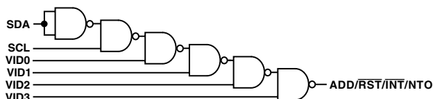
Figure 7. NAND Tree
