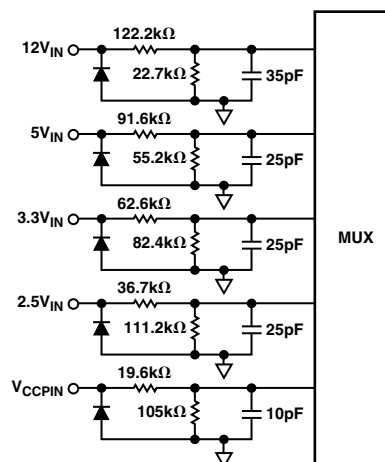
Figure 3. Structure of Analog Inputs
