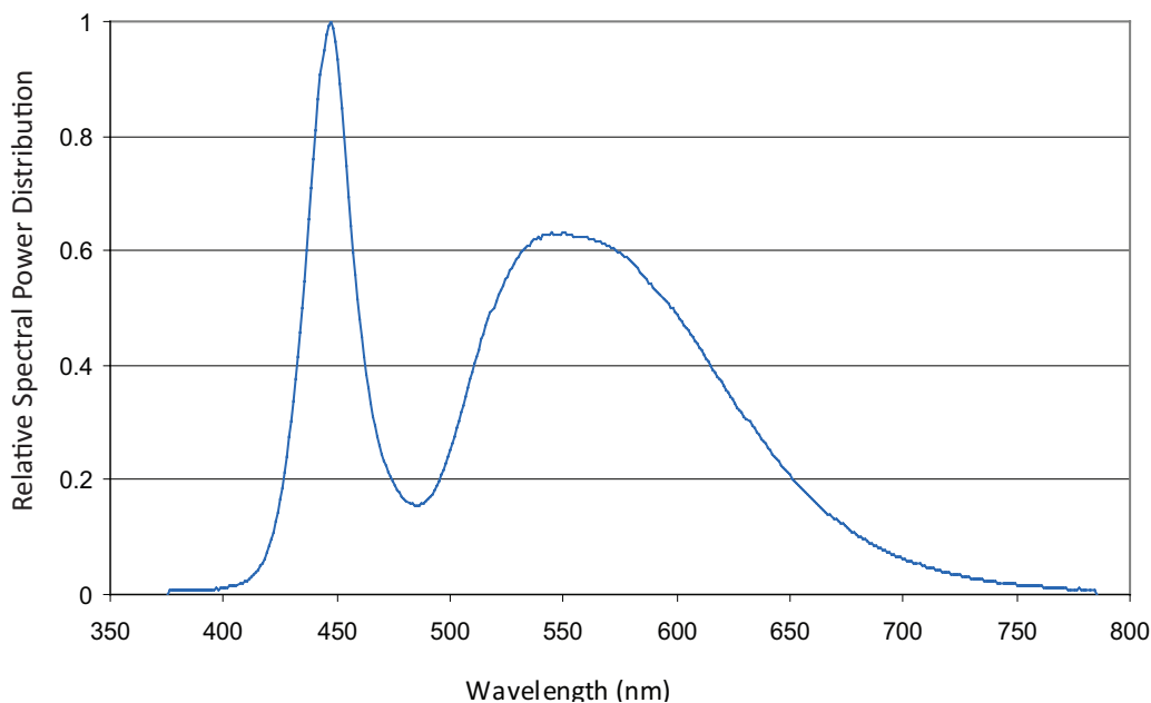
Figure 13. Color spectrum of LXML-PW3I, LXML-PW2I and LXML-PW1I emitters, integrated measurement.
