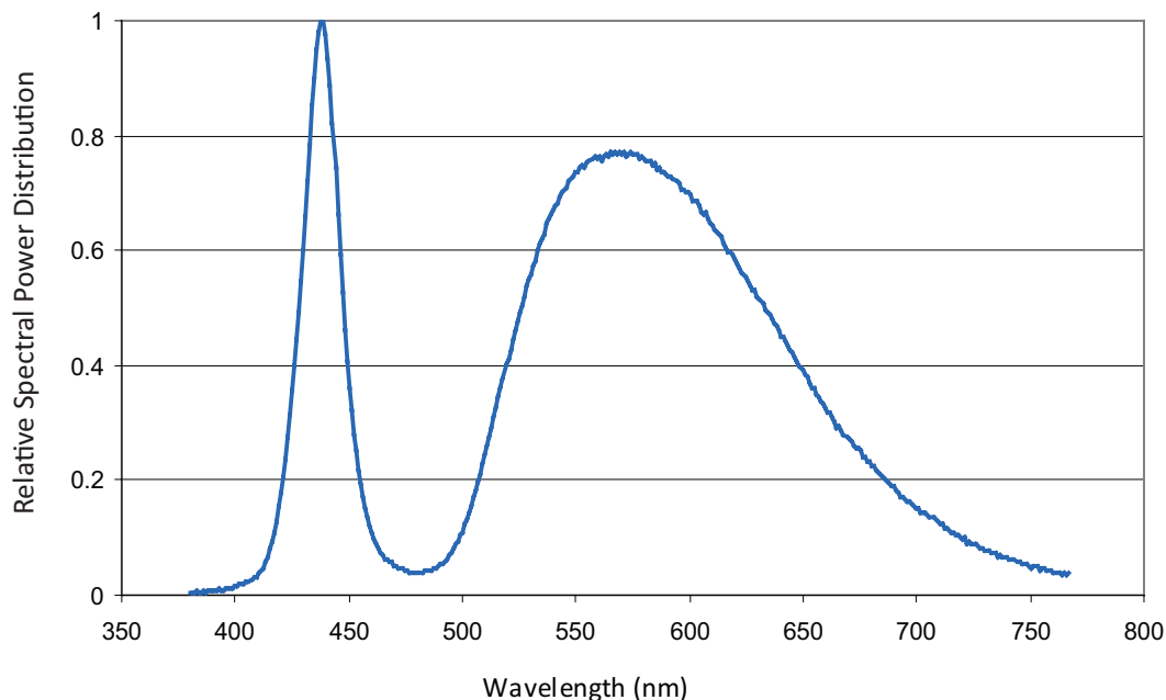
Figure 12. Color spectrum of LXML-PW5I emitter, integrated measurement.
