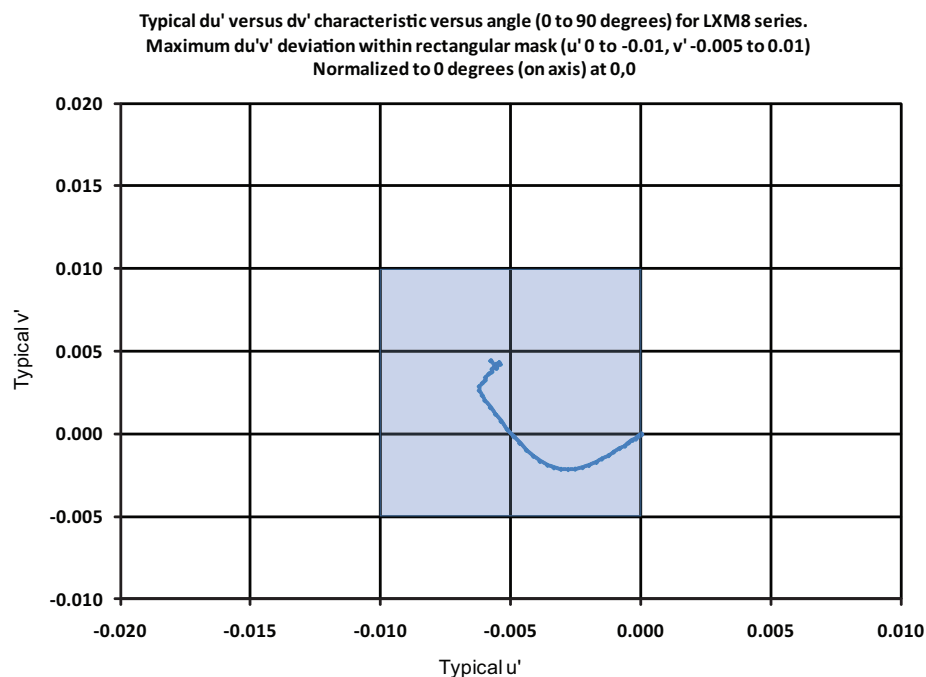
Figure 24. Applicable for LXM8-PW27 and LXM8-PW30 emitters.
