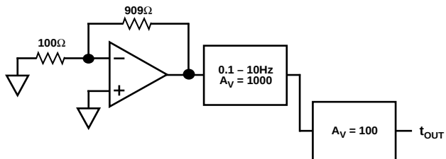
Figure 40. Noise Test Diagram
