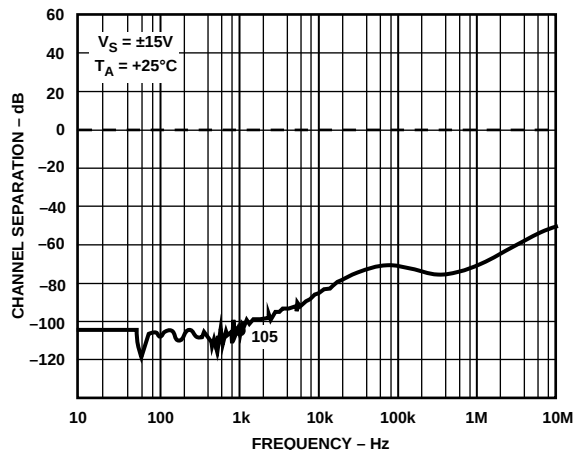
Figure 16. Channel Separation
