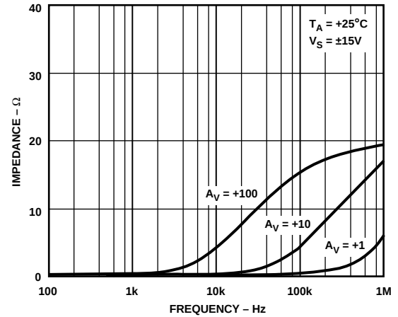
Figure 35. Closed-Loop Output Impedance vs. Frequency @ \pm 15 V
