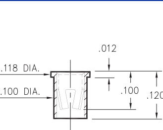
9372-0-15-XX-23-XX-10-0 Solder mount in .102 min. mounting hole
