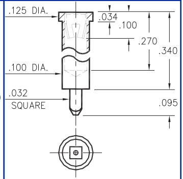
4582-0-15-XX-23-XX-10-0 Square press-fit in .040 plated thru hole
