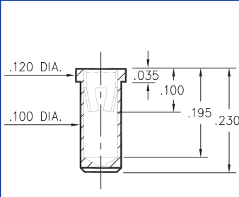
9401-0-15-XX-23-XX-10-0 Solder mount in .102 min. mounting hole Also available on 24mm wide carrier tape: 1,100 parts per 13" reel. Order as: 9401-0-57-XX-23-XX-10-0
