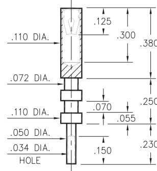
8067-0-19-XX-13-XX-10-0 Wire Termination
