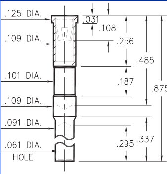
3667-0-19-XX-23-XX-10-0 Wire Termination
