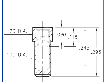
8829-0-15-XX-23-XX-10-0 Solder mount in .102 min. mounting hole
