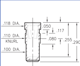
5834-0-15-XX-23-XX-10-0 Press-fit in .107 mounting hole
