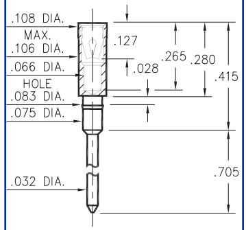
1105-0-15-XX-13-XX-04-0 Press-fit in .080 mounting hole
