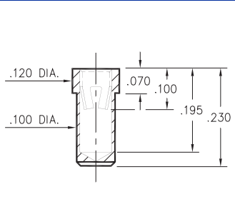
9801-0-15-XX-23-XX-10-0 Solder mount in .102 min. mounting hole Also available on 16mm wide carrier tape: 1,200 parts per 13" reel. Order as: 9801-0-57-XX-23-XX-10-0
