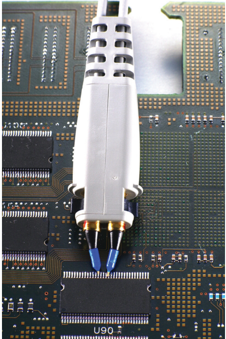
InfiniiMax solder-in probe head with long wires
