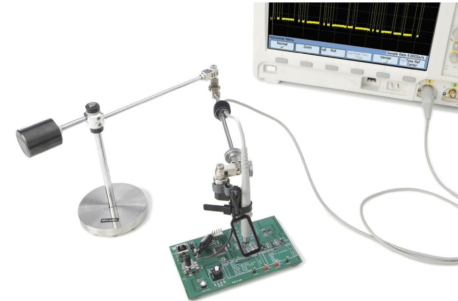
N2784A one-arm probe positioner
