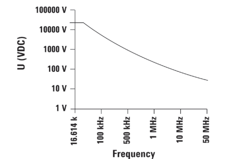
N2771B derating curve
