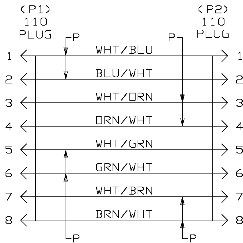
WIRING DIAGRAM
