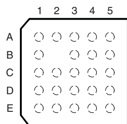
ZQS PACKAGE (TOP VIEW)
