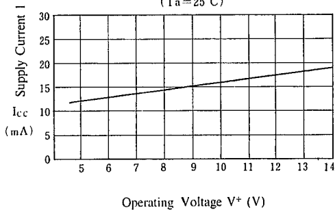
Supply Current 1 vs. Operating Voltage
