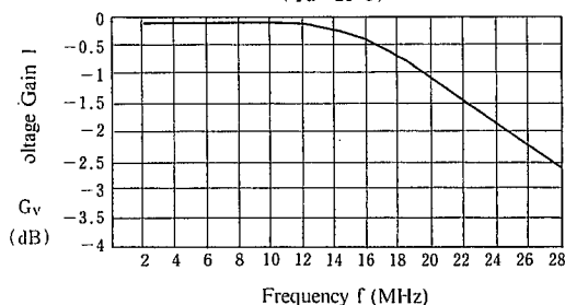
Voltage Gain 1 vs. Frequency
