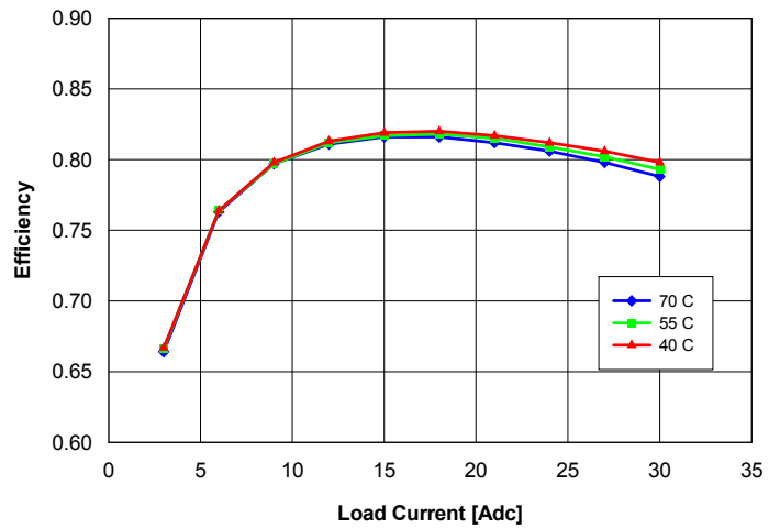
Fig. 14: Efficiency vs. load current and ambient temperature for converter mounted vertically with V_{in} = 54\text{ V} and air flowing from pin 3 to pin 1 at a rate of 200 LFM (1.0 m/s).
