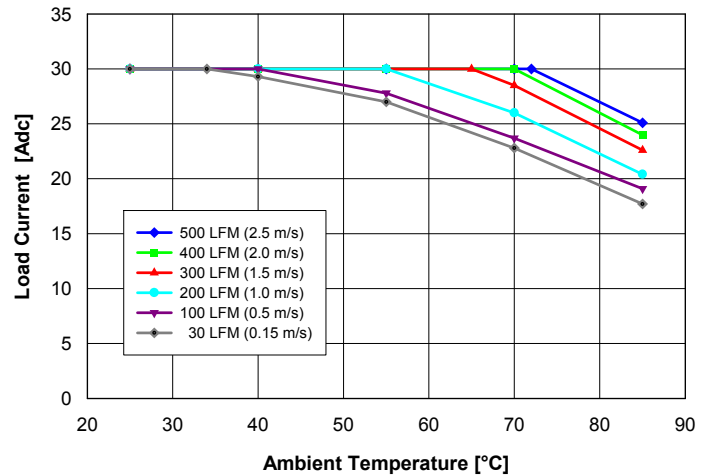
Fig. 10: Available load current vs. ambient air temperature and airflow rates for converter mounted vertically with V_{in} = 54 V, air flowing from pin 3 to pin 1 and maximum FET temperature \leq 105^{\circ}\text{C} .
