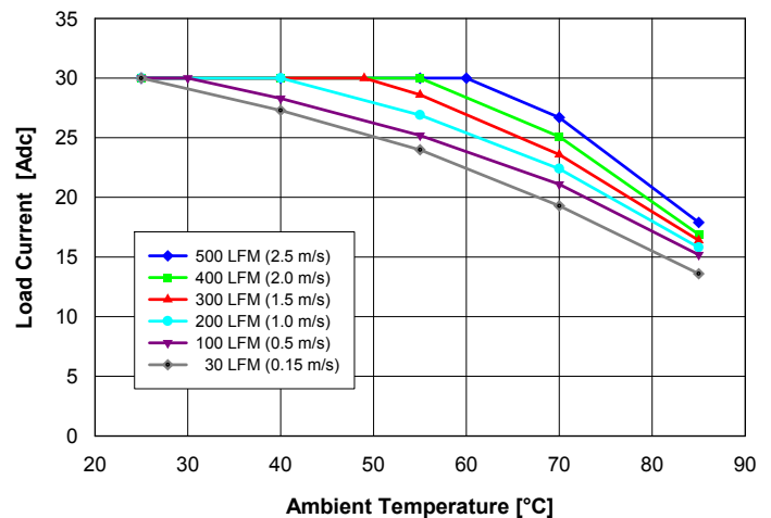
Fig. 12: Available load current vs. ambient temperature and airflow rates for converter mounted horizontally with V_{in} = 54 V, air flowing from pin 3 to pin 4 and maximum FET temperature \leq 105^{\circ}\text{C} .
