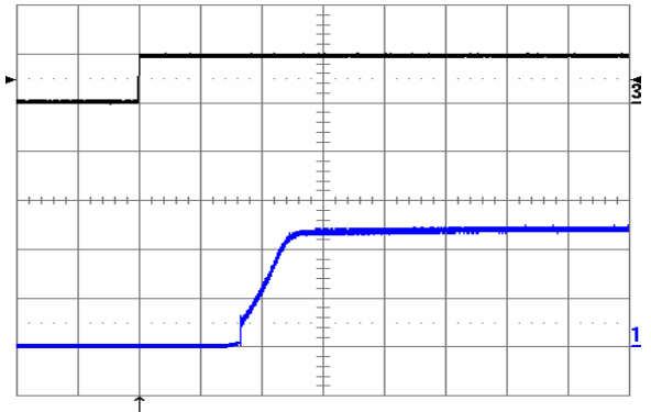
Fig. 18: Turn-on transient at full rated load current (resistive) plus 10,000 \mu\text{F} at V_{in} = 48\text{ V} , triggered via ON/OFF pin. Top trace: ON/OFF signal (5 V/div.). Bottom trace: output voltage (0.5 V/div.). Time scale: 1 ms/div.
