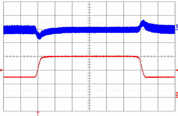
Fig. 19: Output voltage response to load current step-change (7.5 A – 15 A – 7.5 A) at V_{in} = 48\text{ V} . Top trace: output voltage (100 mV/div.). Bottom trace: load current (5 A/div.). Current slew rate: 0.1 A/ \mu\text{s} . C_o = 1\text{ }\mu\text{F} ceramic. Time scale: 0.2 ms/div.
