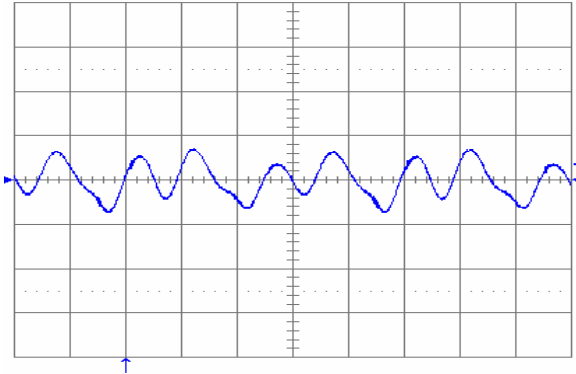
Fig. 21: Output voltage ripple (20 mV/div.) at full rated load current into a resistive load with C_o = 10 \mu\text{F} tantalum + 1\mu\text{F} ceramic and V_{in} = 48 \text{ V} . Time scale: 1 \mu\text{s}/\text{div} .
