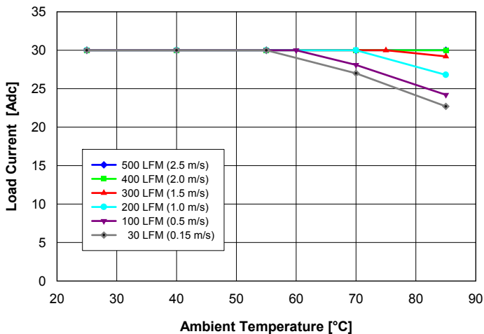
Fig. 1: Available load current vs. ambient air temperature and air-flow rates for QL48T30012 converter mounted vertically with air flowing from pin 3 to pin 1, MOSFET temperature \leq 120^{\circ}\text{C} , V_{in} = 54\text{ V} .
