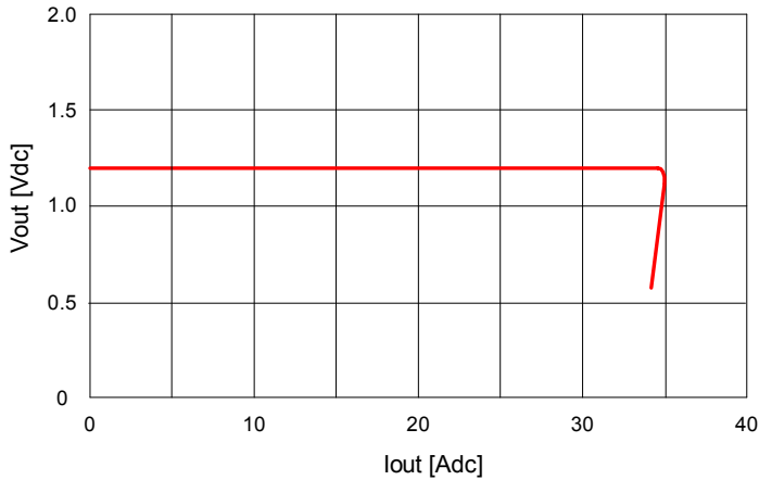
Fig. 25: Output voltage vs. load current showing current limit point and converter shutdown point. Input voltage has almost no effect on current limit characteristic.
