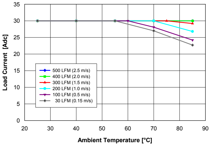
Fig. 9: Available load current vs. ambient air temperature and airflow rates for converter mounted vertically with V_{in} = 54 V, air flowing from pin 3 to pin 1 and maximum FET temperature \leq 120^{\circ}\text{C} .
