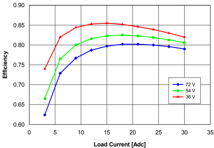
Fig. 15: Efficiency vs. load current and input voltage for converter mounted horizontally with air flowing from pin 3 to pin 4 at a rate of 300 LFM (1.5 m/s) and T_a = 25^\circ\text{C} .
