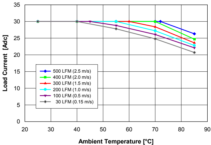
Fig. 11: Available load current vs. ambient temperature and airflow rates for converter mounted horizontally with V_{in} = 54 V, air flowing from pin 3 to pin 4 and maximum FET temperature \leq 120^{\circ}\text{C} .
