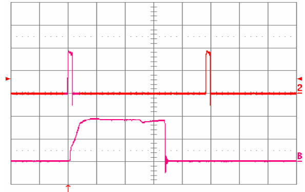
Fig. 26: Load current (top trace, 20 A/div, 20 ms/div) into a 10 mΩ short circuit during restart, at Vin = 48 V. Bottom trace (20 A/div, 1 ms/div) is an expansion of the on-time portion of the top trace.
