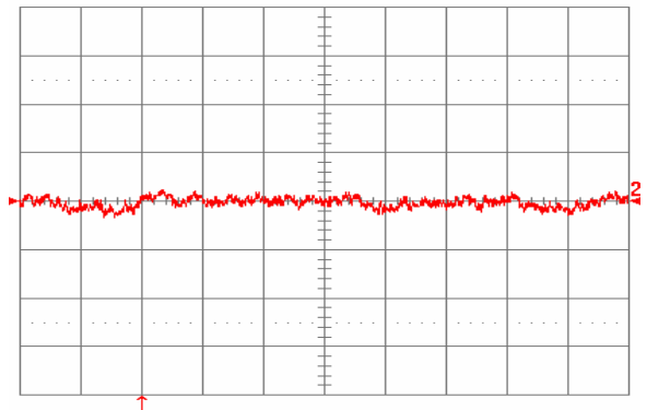
Fig. 24: Input reflected ripple current, i_s (10 mA/div), measured through 10 \mu\text{H} at the source at full rated load current and V_{in} = 48 \text{ V} . Refer to Fig. 22 for test setup. Time scale: 1 \mu\text{s}/\text{div} .
