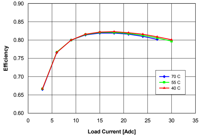
Fig. 16: Efficiency vs. load current and ambient temperature for converter mounted horizontally with V_{in} = 54\text{ V} and air flowing from pin 3 to pin 4 at a rate of 200 LFM (1.0 m/s).
