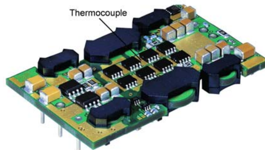
Fig. 27: Location of the thermocouple for thermal testing.
