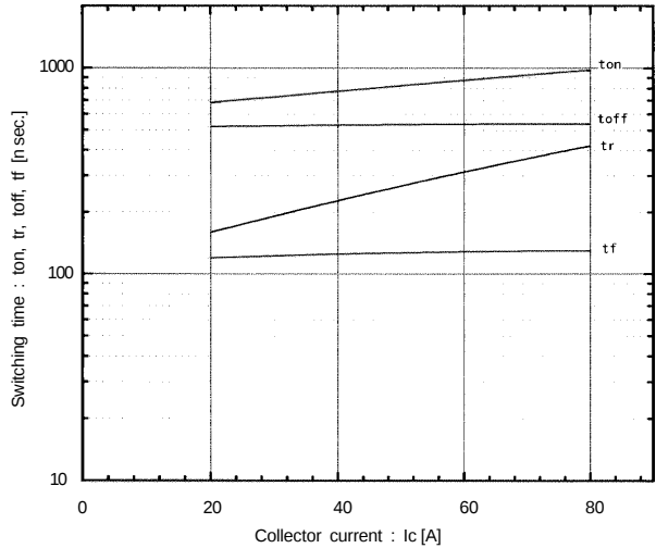
Switching time vs. Collector current V_{CC}=300\text{V} , R_G=62\text{ ohm} , V_{GE}=\pm 15\text{V} , T_j=25^{\circ}\text{C}
