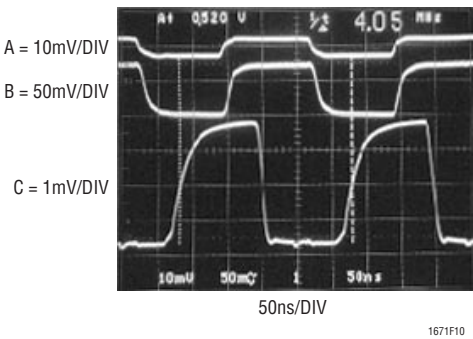
Figure 10. Adaptive Trigger Responding to a 4MHz, 5mV Input. Input Amplitude Variations from 2mV to 175mV Are Accommodated
