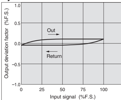
Hysteresis
