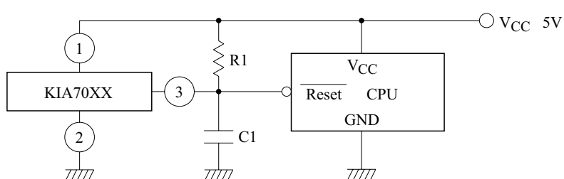
(2) CPU RESETTNG
