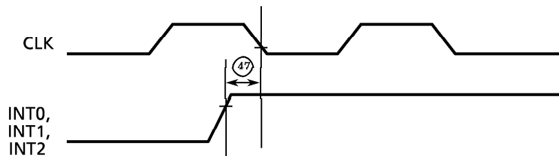
Figure 9.6 Interrupt Request Timing Diagram
